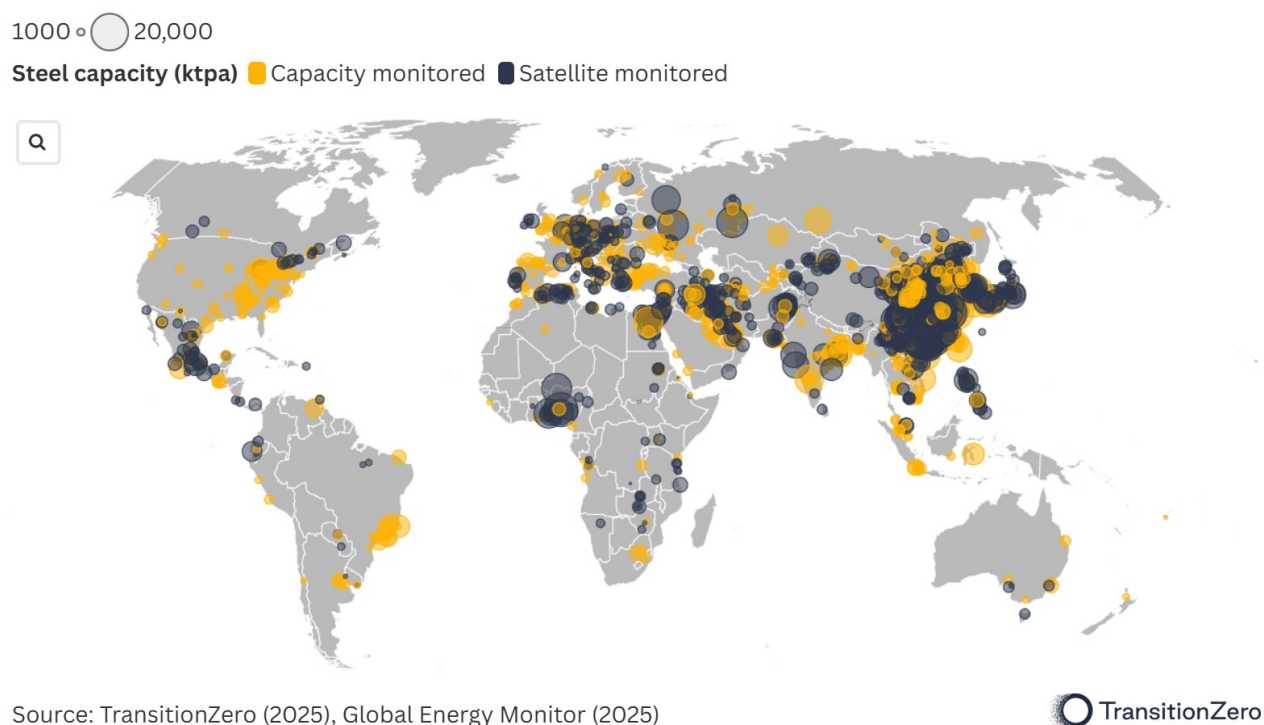
Figure 2 Global map showing operating steel plants as of 2025. Satellite monitored facilities (shown in dark blue) and other facilities (shown in orange). The circle size represents plant production capacity, with reference scales shown at the top of the figure for 1,000 and 20,000 thousand tonnes per annum (ktpa).
