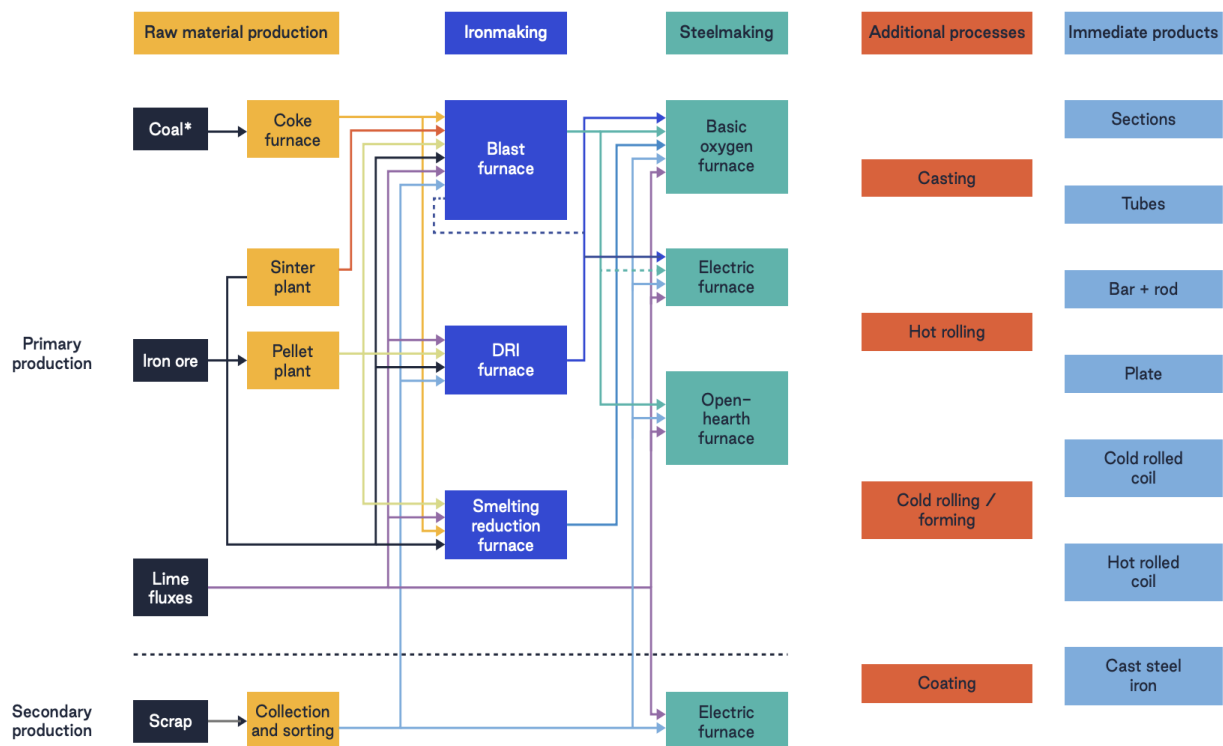
Figure 8 Steel production routes - adapted from IEA (2020).
