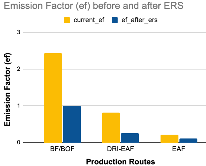
Figure 7 Average emission factors (tCO 2 per tonne of steel) before (yellow bars) and after (blue bars) the application of primary emission reduction solutions (ERS) across major steel production routes worldwide.
