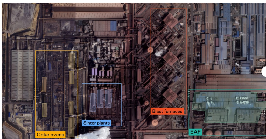
Figure 4 Zooming in on Hyundai Steel Integrated Steel Works (Dangjin, South Korea), with identified sub-asset polygons.
