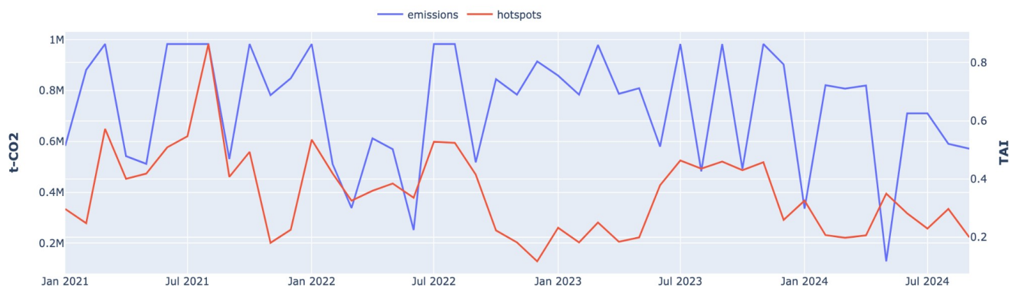
Figure 5 Satellite-based Thermal Anomaly Index (TAI; red solid line) and estimated emissions (blue solid line) at ArcelorMittal’s Fos-sur-Mer steel plant during January 2021– September 2024.
