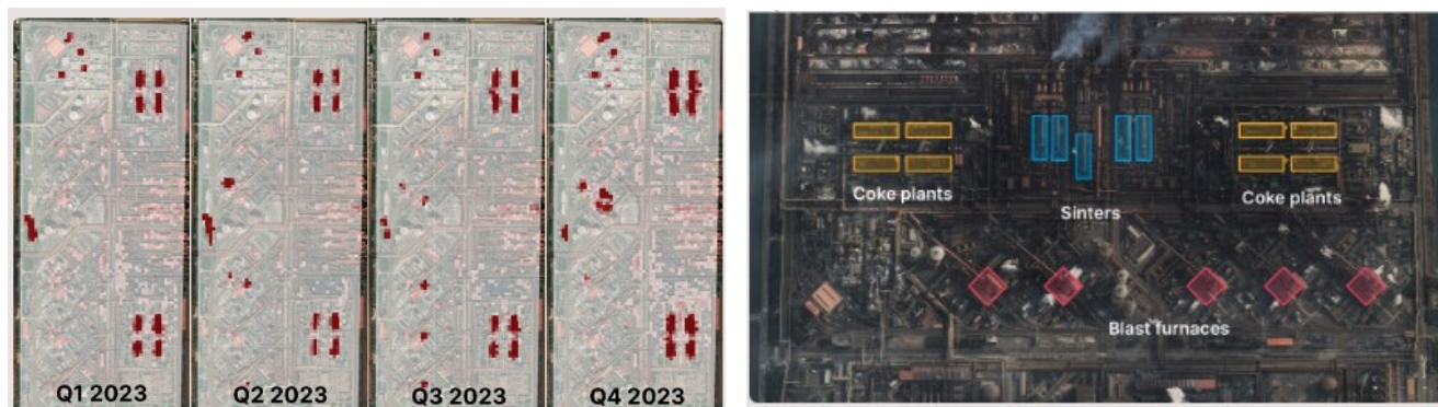
Figure 3 Left: Identified hotspots at POSCO's Gwangyang steel plant, South Korea, during different quarters in 2023. Right: Identified sub-assets within the facility based on thermal anomalies. Sources: modified Copernicus and USGS data, ESRI base map.
