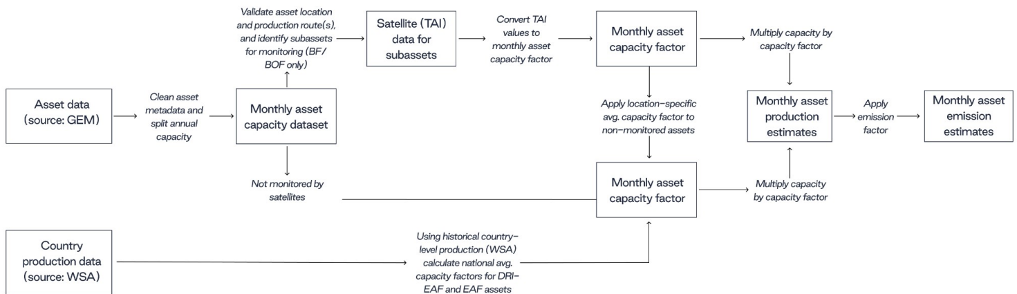
Figure 1 Flowchart of the methodology to calculate plant-level emissions for global steel assets.
